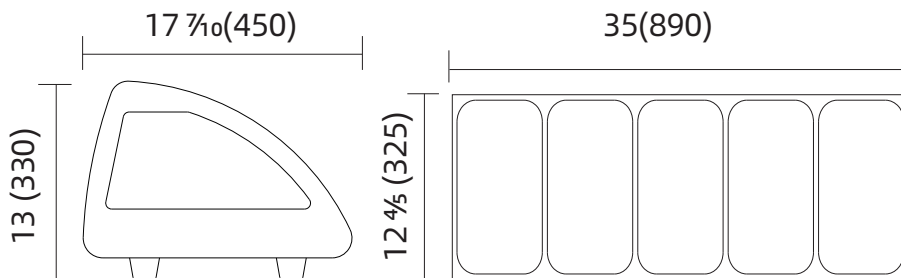
5x1/3 GN plate
